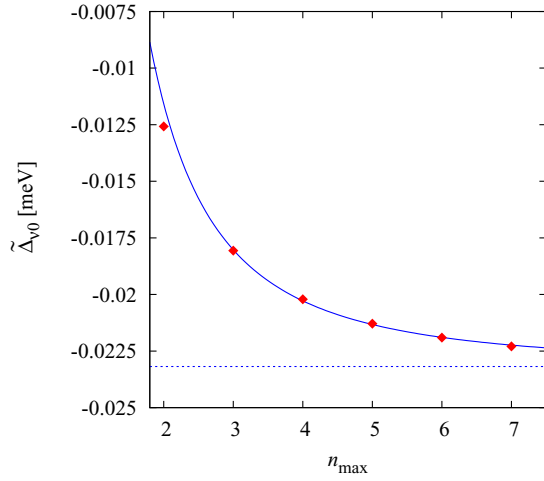
FIG. 1. In order to evaluate the quantities \Gamma_{v_2 v_1 \mathbf{0}}(\omega) and \Delta_{v_2 v_1 \mathbf{0}}(\omega) , one has to cut the infinite sums over \nu in the formulas at a finite value n_{\max} of the principal quantum number n [cf. Eq. (16)]. Here we show the values obtained for \tilde{\Delta}_{210\mathbf{0}} in dependence on n_{\max} for Step 2. The final value \tilde{\Delta}_{210\mathbf{0}} = -2.32 \times 10^{-5} eV (dashed line) is then calculated from an extrapolation. We used f(n_{\max}) = a/n_{\max}^2 + b as a fitting function for n_{\max} \geq 3 (solid line).
