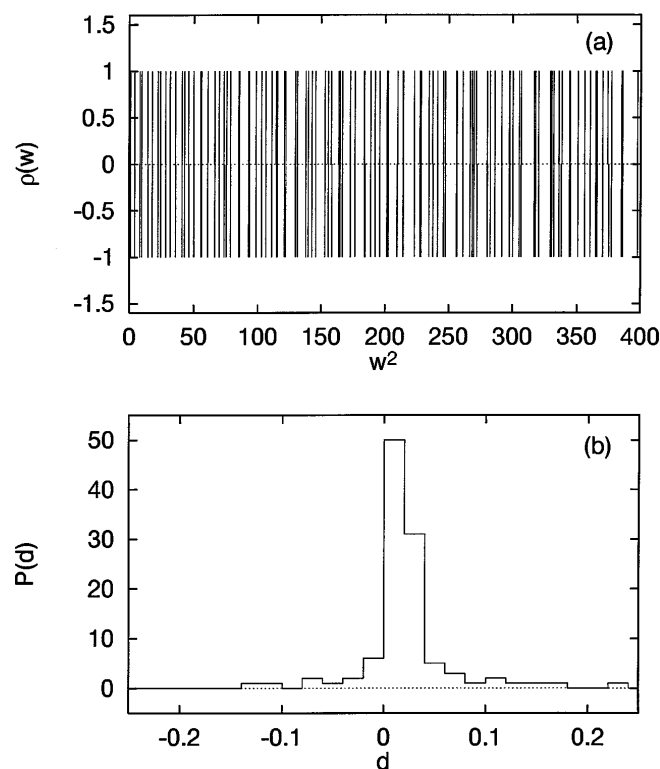
FIG. 3. (a) Semiclassical (upper part) and quantum mechanical (lower part) spectrum of the hydrogen atom in a magnetic field at scaled energy \tilde{E} = -0.4 . (b) Distribution P(d) of the semiclassical error in units of the mean level spacing, d = (w_{\text{qm}} - w_{\text{sc}})/\Delta w_{\text{av}} for the lowest 106 eigenvalues.
