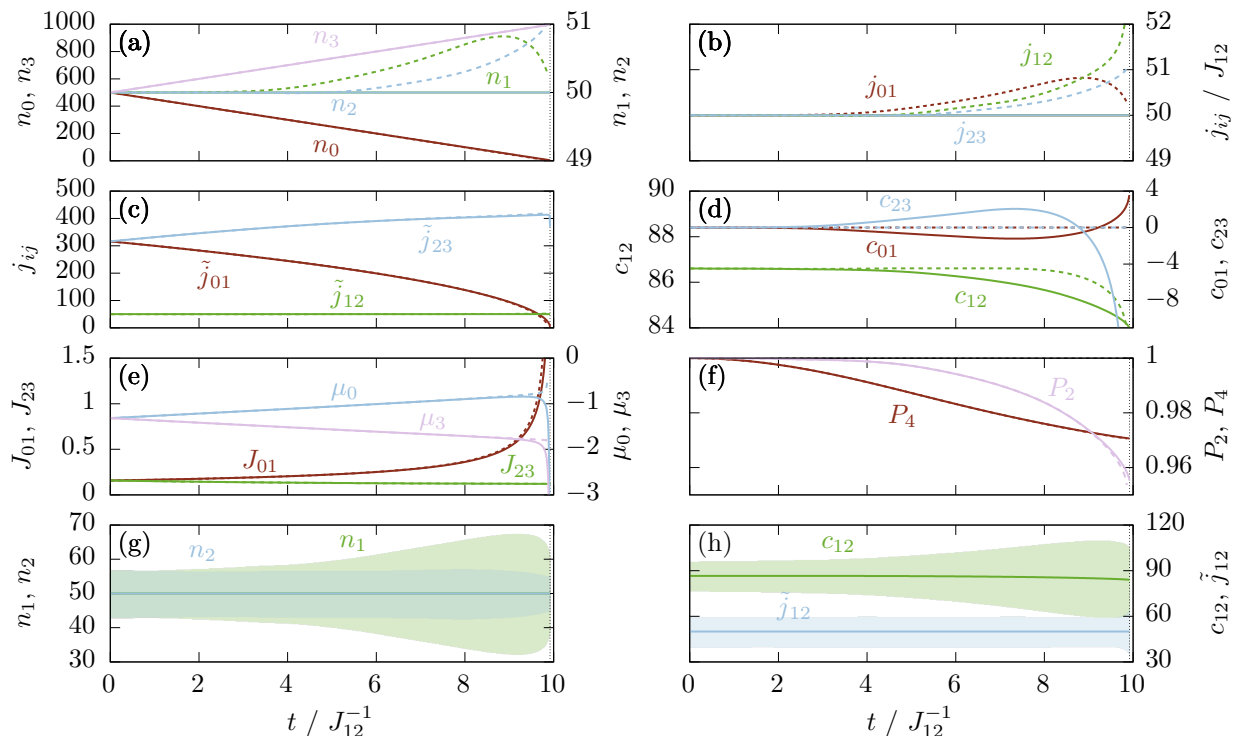
FIG. 5. Comparison of the first approach from Fig. 2 (dashed lines) with the second approach from Fig. 4 (solid lines) for a total number of 1100 particles with the same occupation ratio as before. Many-body calculations were performed within the BBR approximation. Although the time of the breakdown (dotted vertical line) almost matches that of the MF limit in Figs. 2 and 4 (note that the calculation ends slightly before t = 10 ), there are still deviations from the MF dynamics (a–d), cf. Figs. 2 and 4. For both approaches the time-dependent parameters are in good agreement and only show different behavior close to the breakdown. The same holds for the purities of the four-mode system P_4 and the embedded two-mode system P_2 (f). The standard deviations for the embedded observables are shown for the BGL state (g–h). Note that Figs. (a), (d), and (e) have two separate vertical axes due to the different ranges of their observables.
