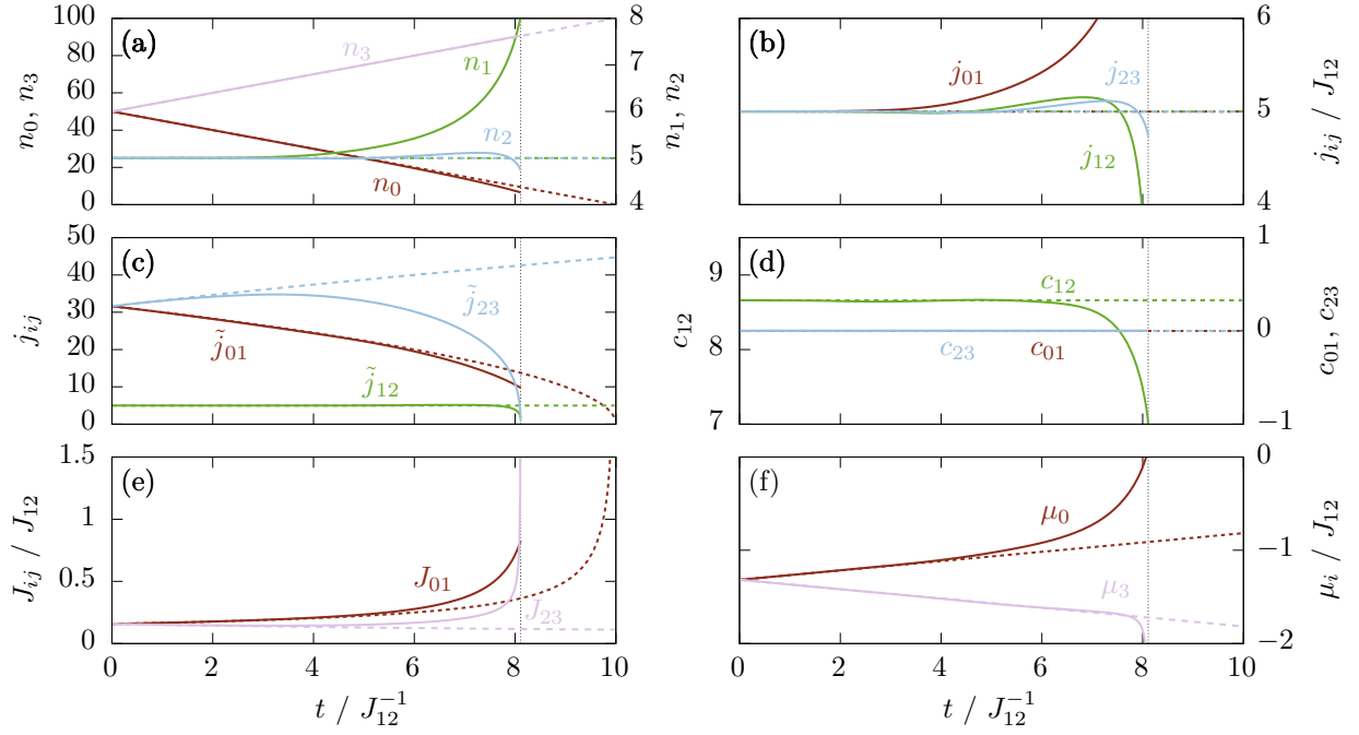
FIG. 2. Observables and parameters for a weakly interacting BEC with g = 0.1 described by the BH model. The coupling strength is fixed to \gamma = 0.5 and the occupation ratio between the embedded system and the reservoir is 10 for a total number of N = 110 particles. In comparison with the MF limit (dashed lines), the many-body system (solid lines) shows no quasi-stationary behavior, which is clearly visible by looking at the occupation numbers n_1 and n_2 (a), and the reduced current \tilde{j}_{12} (b) and c_{12} (d). The many-body calculations also show an earlier breakdown of the system (dotted vertical line) due to \tilde{j}_{23} dropping to zero (c), leading to divergent tunneling rates (e) and on-site energies (f). Note that Figs. (a) and (d) have two separate vertical axes due to the different ranges of their observables.
