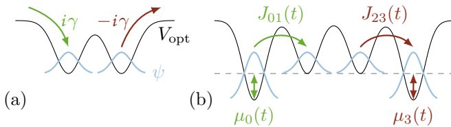
FIG. 1. Open non-Hermitian two-mode system (a) and closed Hermitian four-mode system (b). The currents between the outer reservoir wells and the inner wells account for the in- and out-coupling of particles in the open quantum system. To reproduce the properties of an open system the additional parameters J_{01}(t) , J_{23}(t) , \mu_0(t) and \mu_3(t) have to be varied time-dependently.
