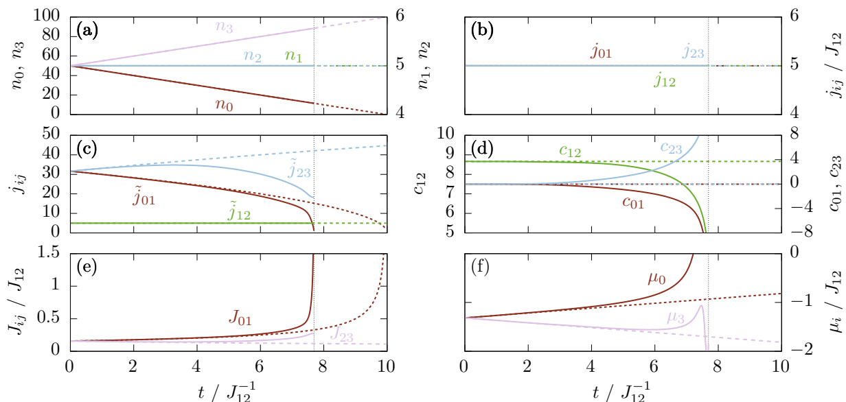
FIG. 4. Same as Fig. 2 but with modified on-site energies as shown in Fig. 3. The BH dynamics (solid lines) show stationary occupation numbers (a) in the embedded wells and stationary currents (b) between neighboring wells, which we call the BGL state. There is still an earlier breakdown in comparison with the MF dynamics (dashed lines), now caused by \tilde{j}_{01} dropping to zero. Due to the modifications (33), some parameters are no longer monotonous (f). Note that Figs. (a) and (d) have two separate vertical axes due to the different ranges of their observables.
