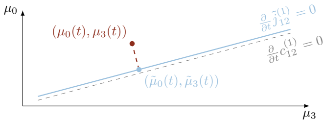
FIG. 3. Eqs. (31) in the vicinity of pure states. Since both lines are almost parallel, the unique solution cannot be calculated accurately. By projection of the parameters (30) onto the imaginary part yielding (\tilde{\mu}_0, \tilde{\mu}_3) a constant particle flow between the inner wells is achieved. While in principle all points on the solid curve representing Eq. (31b) are valid, our approach stays as close as possible to the former approach adapted from the MF.
