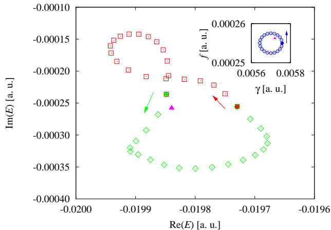
FIG. 2: (Color online) Paths of the two eigenvalues (represented by squares and diamonds, respectively) which degenerate at the exceptional point labeled 14 in Table I in the complex energy plane [40]. Each point of one eigenvalue belongs to a different set of parameters. The path in the field strength parameter space is a circle defined in Eq. (14) with \delta = 0.01 (see inset). The initial set of parameters and the corresponding eigenvalues are represented by filled starting points. The arrows indicate the direction of progression. The filled triangle marks the position of the exceptional point in the parameter space and the corresponding complex energy of the degenerate resonances.
