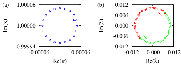
FIG. 1: (Color online) (a) Circle in the parameter space \kappa with the exceptional point \kappa_+ = i as center point for the simple model (1). (b) Eigenvalues \lambda_{1,2} calculated for the parameter values from (a) indicated by red squares and green diamonds, respectively. In this case each of the two eigenvalues traverses a semicircle. In (a) and (b) the filled symbols represent the first parameter value \kappa_0 and the corresponding eigenvalues \lambda_{1,2}(\kappa_0) , respectively. The arrows point in the direction of progression.
