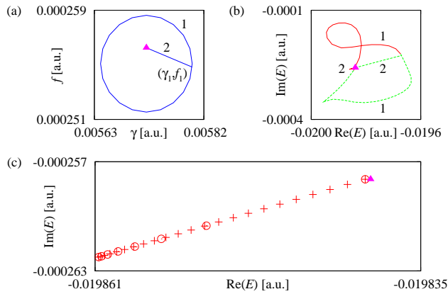
FIG. 4: (Color online) (a) A circle in the parameter space (labeled 1) is chosen such that it passes through the parameter set (\gamma_1, f_1) at which one of the energy eigenvalues is identical with its position at the exceptional point. A straight line (labeled 2) connects the parameters of the exceptional point and the parameter set (\gamma_1, f_1) . (b) Paths of the two numerically exact complex energies for the circle and the straight line described in (a). (c) Magnification of the path of the eigenvalue denoted by the red solid line in (b) for the parameter line labeled 2 in (a). The eigenvalue departs from the point of degeneracy (circles) and returns to its initial value (plus symbols).
