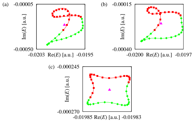
FIG. 3: (Color online) Paths of the two eigenvalues considered in Fig. 2 for different radii of the parameter space circle (14), where the center (\gamma_0, f_0) = (\gamma^{(\text{EP})}, f^{(\text{EP})}) was always chosen to be exactly the exceptional point. (a) \delta = 3 \times 10^{-2} , (b) \delta = 10^{-2} , (c) \delta = 10^{-4} . The position of the resonances at (\gamma^{(\text{EP})}, f^{(\text{EP})}) is marked by a triangle in each figure. The squares and diamonds represent the exact quantum resonances. The lines represent the eigenvalues of the two-dimensional matrix model (15), whose coefficients have been fitted to the numerical results of the exact quantum calculations.
