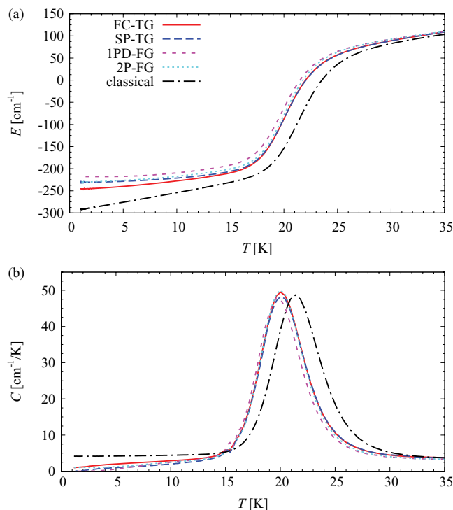
FIG. 3. Mean energy (a) and specific heat (b) of the argon trimer calculated with the Gaussian approximations FC-TG, SP-TG, 1PD-FG, 2P-FG, and classically for R_c = 32 \text{ \AA} .
