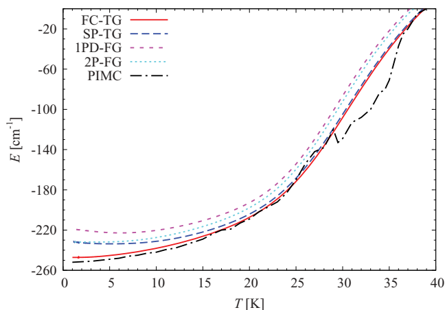
FIG. 2. Comparison of the mean energy obtained with the Gaussian methods FC-TG, SP-TG, 1PD-FG, and 2P-FG with the path-integral Monte Carlo (PIMC) values taken from Ref. 6. The kinetic energy of the free center of mass motion is subtracted from our results to allow for the comparison.
